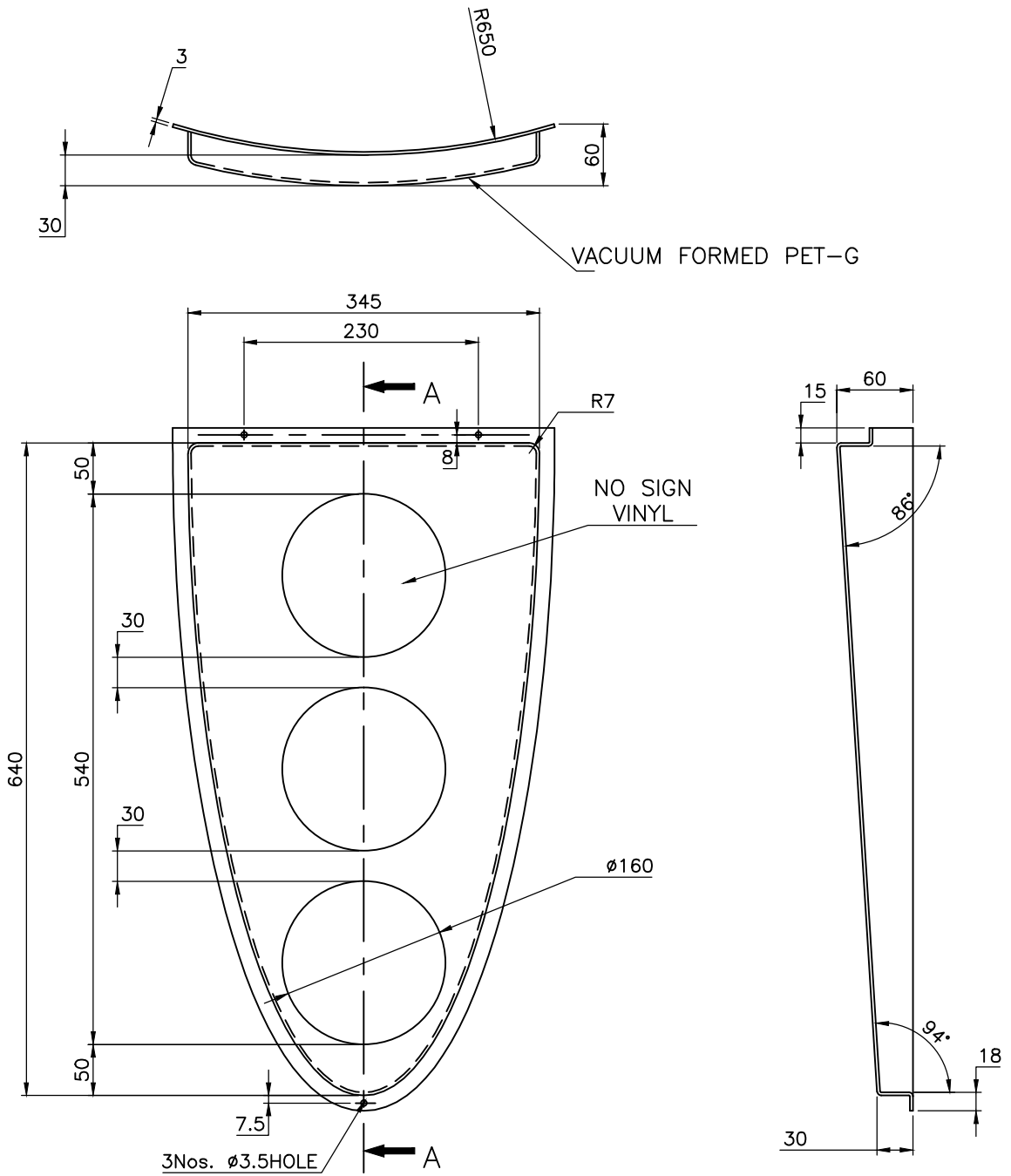
SECTION AA
